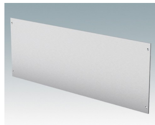
M6400706 Front Panel 312 Aluminum Matt anodized 12.68"x0.08"x4.56"
