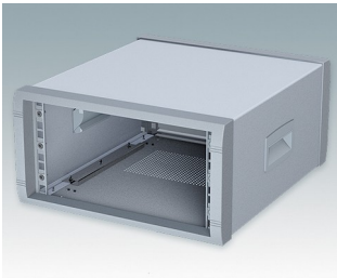
M6010305 INSTRUMET 10.5" 3Ux13.78" Aluminum Light gray/window gray RAL 7035/7040 6.18"x11.93"x13.78"
