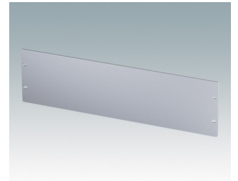
M6019001 Front panel 3Ux19" Aluminum Matt anodized 19.00"x0.12"x5.22"
