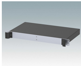
M6219119 COMBIMET 19" 1Ux10.43" Solid Top Aluminum Black RAL 9005 1.72"x19.00"x10.43"
