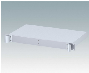
M6219115 COMBIMET 19" 1Ux10.43" Solid Top Aluminum Light gray RAL 7035 1.72"x19.00"x10.43"
