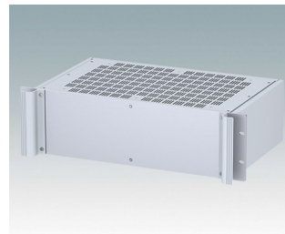
M6219345 COMBIMET 19" 3Ux10.43" Vented Aluminum Light gray RAL 7035 5.22"x19.00"x10.43"
