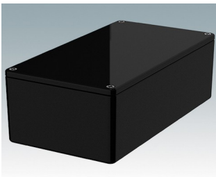
5005-15-BLK Diecast Enclosure Diecast Aluminum Black RAL 9004 5.98"x3.23"x1.97" IP 65 opt.
