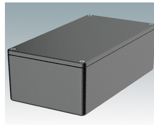
5005-15-PAT Diecast Enclosure Diecast Aluminum Hammer tone 5.98"x3.23"x1.97" IP 65 opt.
