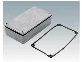
FT094-509 Sealing Gasket (NEMA 4) Rubber Black IP 65
