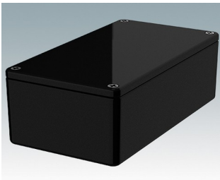
5004-14-BLK Diecast Enclosure Diecast Aluminum Black RAL 9004 4.72"x2.60"x1.57" IP 65 opt.
