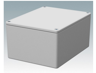
5007-17-WH Diecast Enclosure Diecast Aluminum Pure white RAL 9010 4.76"x3.74"x2.40" IP 65 opt.
