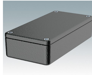
5002-12-PAT Diecast Enclosure Diecast Aluminum Hammer tone 3.98"x1.97"x0.98" IP 65 opt.
