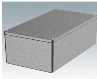
5005-15-NAT Diecast Enclosure Diecast Aluminum Natural finish 5.98"x3.23"x1.97" IP 65 opt.
