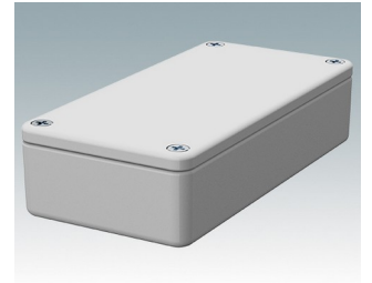
5002-12-WH Diecast Enclosure Diecast Aluminum Pure white RAL 9010 3.98"x1.97"x0.98" IP 65 opt.
