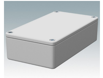
5003-13-WH Diecast Enclosure Diecast Aluminum Pure white RAL 9010 4.41"x2.44"x1.20" IP 65 opt.
