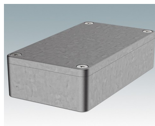
5500-06 Sealed Diecast Enclosure Diecast Aluminum Natural finish 4.53"x2.56"x1.18" IP 65
