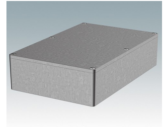
5500-24 Sealed Diecast Enclosure Diecast Aluminum Natural finish 8.74"x5.75"x2.17" IP 65
