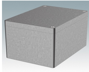
5500-15 Sealed Diecast Enclosure Diecast Aluminum Natural finish 5.83"x4.25"x2.95" IP 65
