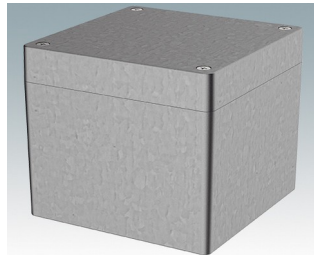
5500-37 Sealed Diecast Enclosure Diecast Aluminum Natural finish 4.76"x4.76"x3.98" IP 65
