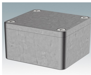
5500-04 Sealed Diecast Enclosure Diecast Aluminum Natural finish 2.52"x2.28"x1.38" IP 65
