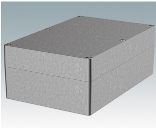
5500-25 Sealed Diecast Enclosure Diecast Aluminum Natural finish 8.74"x5.71"x3.23" IP 65
