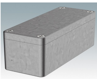
5500-02 Sealed Diecast Enclosure Diecast Aluminum Natural finish 3.54"x1.42"x1.18" IP 65
