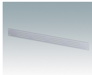
M6019011 Front panel 1Ux19" vented Aluminum Matt anodized 19.00"x0.12"x1.72"
