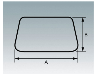
M0000805 D-SUB Cutout Punch Tools
